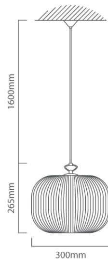
P930 CAD DIAGRAM
