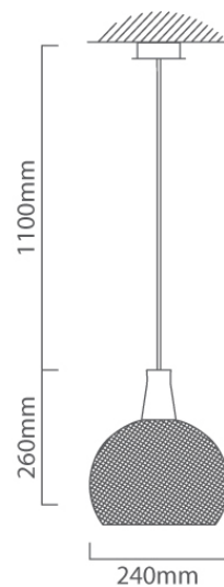
P936 CAD DIAGRAM
