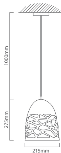
P941 CAD DIAGRAM
