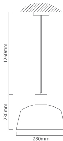
P966 CAD DIAGRAM
