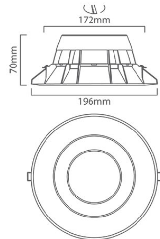
PR203 CAD DIAGRAM
