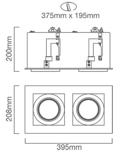
PR338 CAD DIAGRAM
