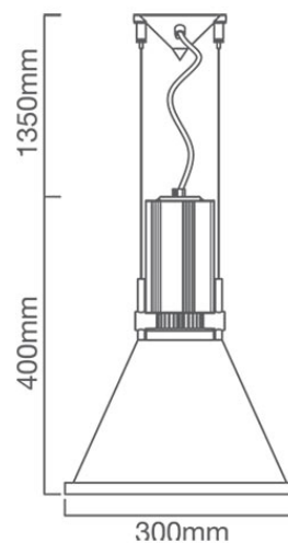
PR366 CAD DIAGRAM
