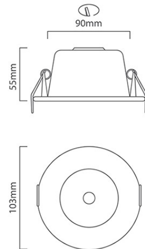
PR456 CAD DIAGRAM
