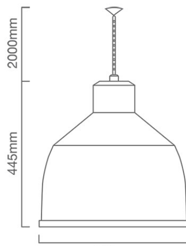
PR48 CAD DIAGRAM
