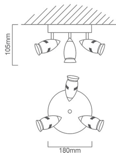
S222 CAD DIAGRAM
