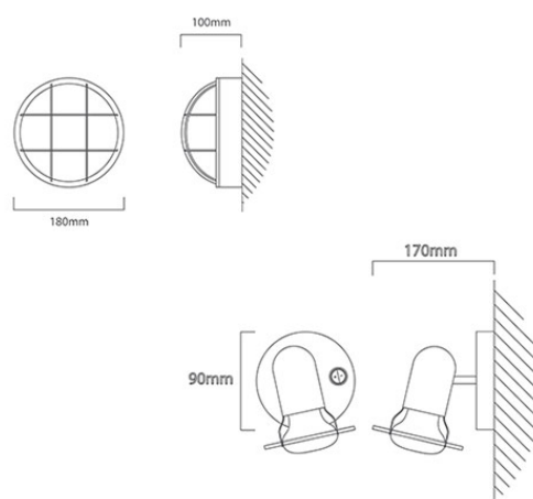
S242 CAD DIAGRAM
