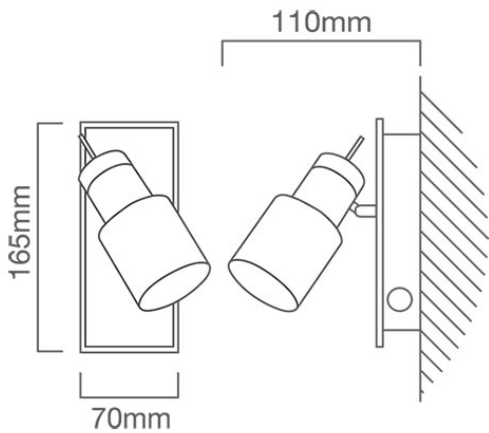
S371 CAD DIAGRAM
