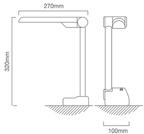
T18 CAD DIAGRAM
