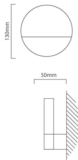
W170 CAD DIAGRAM
