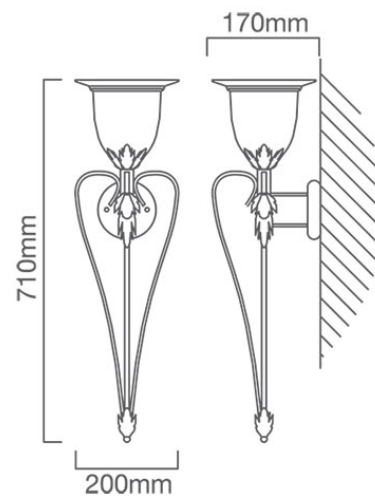
W299 CAD DIAGRAM
