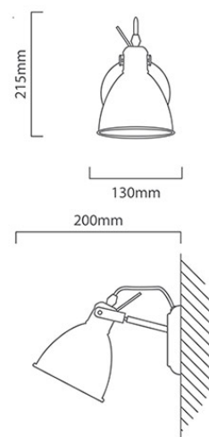
W494 CAD DIAGRAM
