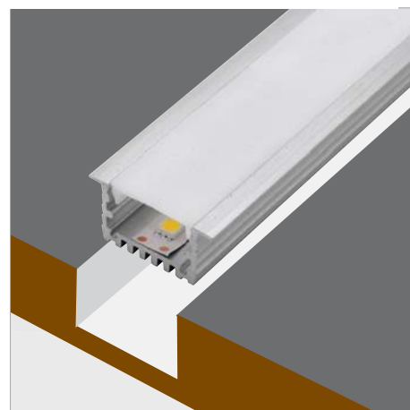
Make the necessary cut out and and install the Zero Recessed
